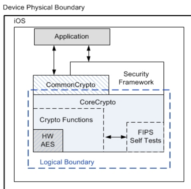
Figure 3: Logical Block Diagram of the Apple CoreCrypto Module v8 for ARM.
