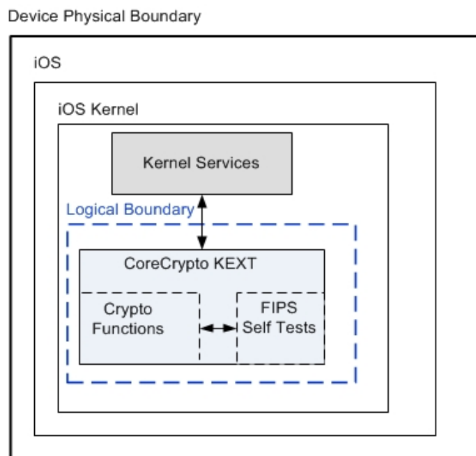
Figure 2: Logical Block Diagram of the Apple CoreCrypto Kernel Module v8 for ARM
