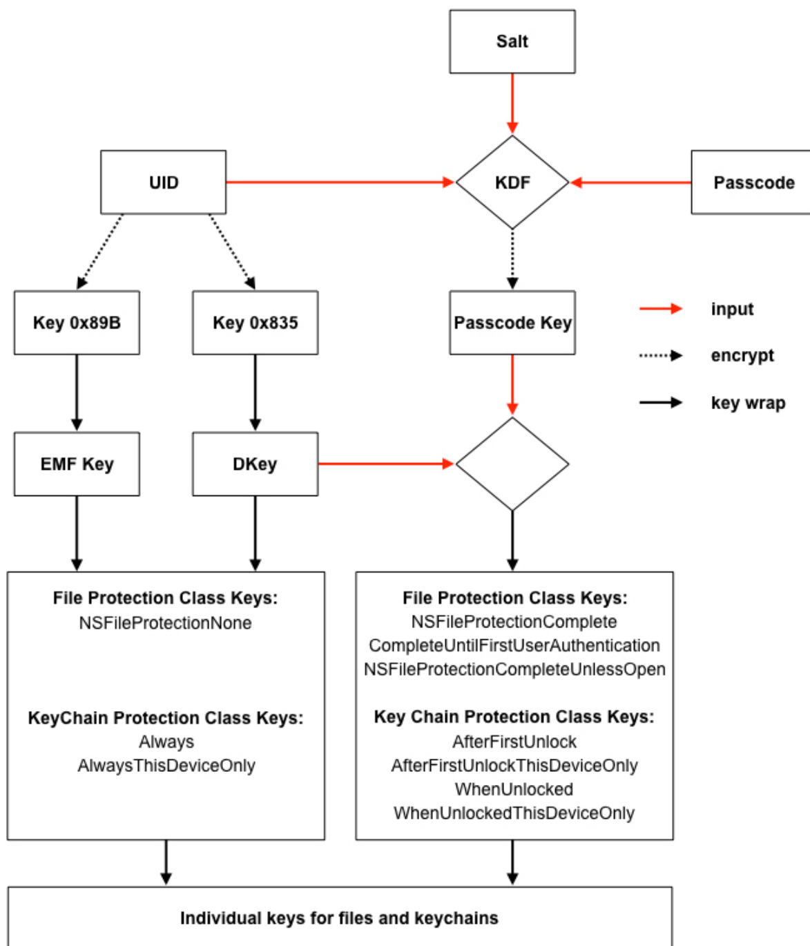
Figure 4: Key Hierarchy in iOS
